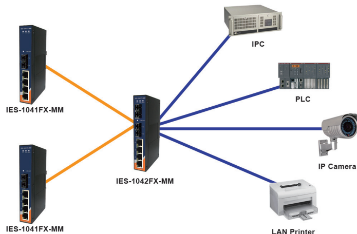
Connections of Ethernet devices
