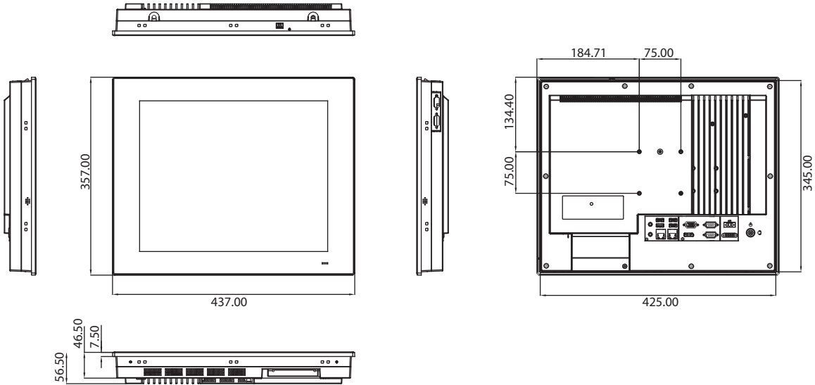
Panel Cutout Dimensions: 427 x 347 mm (16.81 x 13.66 in)
